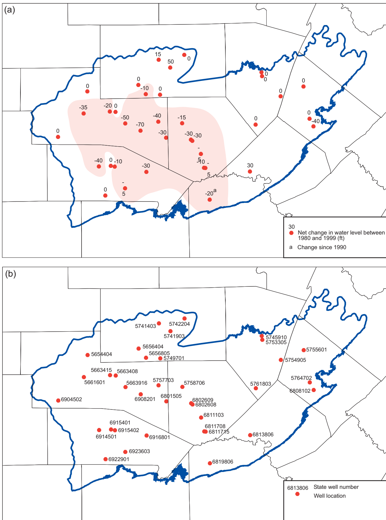
Figure 24. (a) Net change in water level in the Middle Trinity aquifer between 1980 and 1999. (b) State well number for the analyzed wells.
